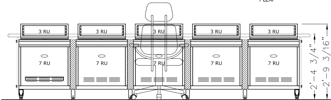
FRONT ELEVATION
