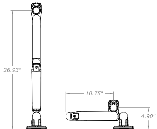
PLAN VIEW A
